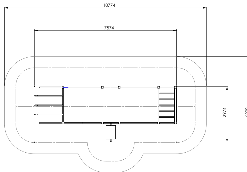
MOVEMENT RIG
